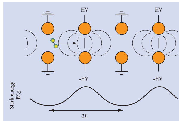
Fig. 2: Scheme of the Stark decelerator, together with the Stark energy of a molecule as a function of position z along the molecular beam axis. In our prototype set-up there are 64 electric field stages separated by a distance L = 5,5 mm. Each stage consists of two parallel cylindrical metal rods with 3 mm diameter centered 5 mm apart. One of the rods is connected to a positive and the other to a negative switchable high voltage power supply. Typically, the decelerator is operated at voltages of +10 kV and -10 kV, leading to a maximum electric field on the molecular beam axis of 90 kV/cm. The maximum Stark shift for ND 3 molecules in the particular low-field seeking quantum state that is selected in these experiments is then 1.1 cm -1 . Close to the electrodes, the electric field is 120 kV/cm, leading to a focusing of the molecules in low-field seeking states towards the molecular beam axis.
