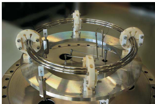
Photograph of the 25 cm diameter hexapole torus, the prototype storage ring for neutral polar molecules.
