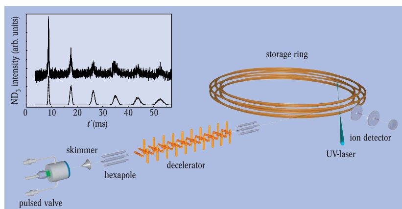
Fig. 3: Schematic view of the experimental setup used for demonstrating the prototype storage ring for neutral molecules. Bunches of ammonia molecules that exit the Stark decelerator with a forward velocity of 89 m/s and with a velocity spread corresponding to a translational temperature of 10 mK are tangentially injected into the electrostatic storage ring, and pass through the 2 mm wide ‘slit’ between the 4 mm diameter hexapole rods. The density of ammonia molecules at the point at which they are coupled into the 25 cm diameter storage ring is measured using a
