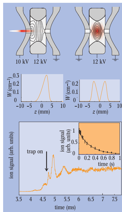
Fig. 4: Electric field configuration used for loading (upper left) and trapping (upper right) neutral polar molecules. In both cases, a cut through the trap is shown and the applied voltages indicated. The solid curves inside the trap are lines of equal electric field. The potential energy along the molecular beam axis for ammonia molecules in the selected low-field seeking state is shown for these two cases as well. In the lower part of the Figure the density of ammonia molecules recorded at the center of the trap is shown as a function of time. The time at which the voltages are switched from the loading to the trapping geometry is indicated with an arrow. After the oscillations in the ammonia density at the center of the trap have faded away, a steady signal of trapped ammonia molecules, corresponding to a density of at least 10^7 molecules per cubic centimeter, remains. The inset shows the density of ammonia molecules on a longer timescale, and an exponential fit to the data with an 1/e decay time of 0.5 s.
